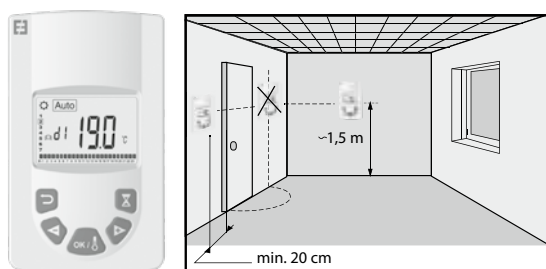
Abb. 97 Funk-Raumthermostat
