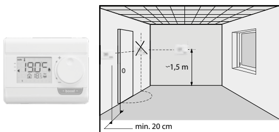
Abb. 102 Funk-Raumthermostat
